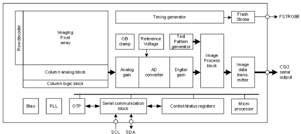
Block Diagram
