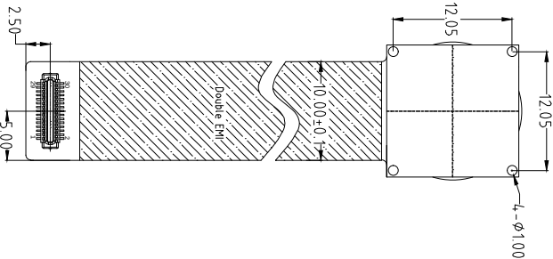
BOTTOM VIEW
